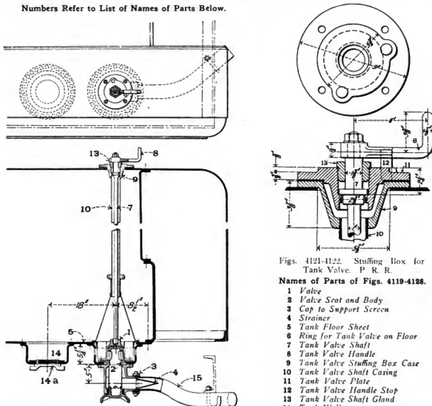
Figs. 4119-4120. General Arrangement of Tank Valve. Pennsylvania Railroad.
